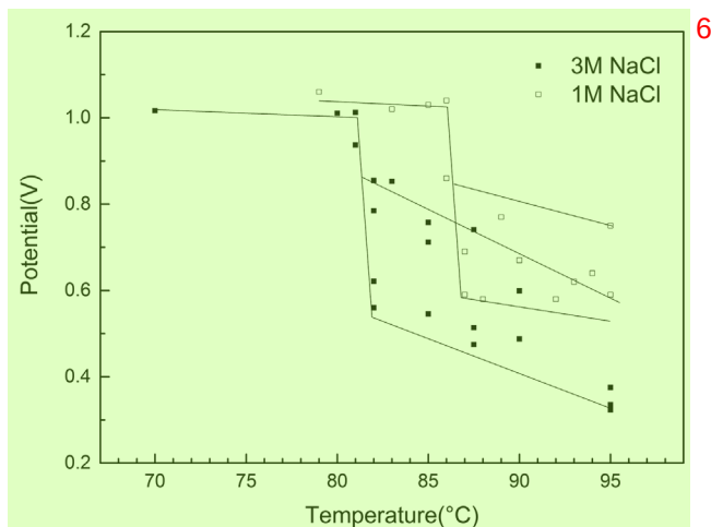
FIGURE 8 Z curves of 254SMO in 1 M and 3 M NaCl 7
