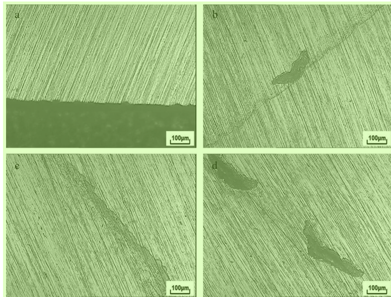
FIGURE 5 Marginal morphology of 317L after cyclic polarization test at lower temperature: (a) before removing the cover, (b–d) after removing the cover
