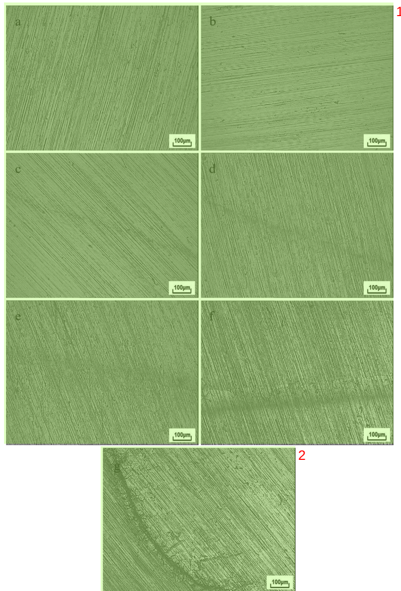
FIGURE 12 Marginal morphology of 904L after potentiostatic polarization test: (a) 800 mV, (b) 850 mV, (c) 900 mV, (d) 950 mV, (e) 1000 mV, (f) 1100 mV, and (g) 1200 mV 3
