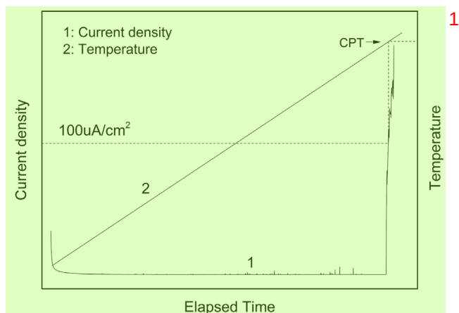
FIGURE 2 Schematic diagram of potentiostatic CPT measurement
