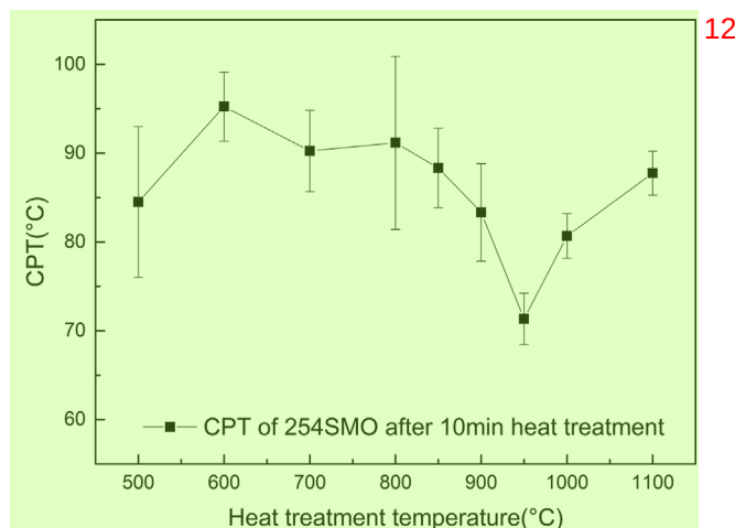
FIGURE 9 Potentiostatic CPT of 254SMO after 10 min heat treatment at different temperatures 13
