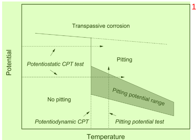
FIGURE 1 Ideal Z curve of austenitic stainless steel (plotting pitting potential or transpassive potential vs. temperature)
