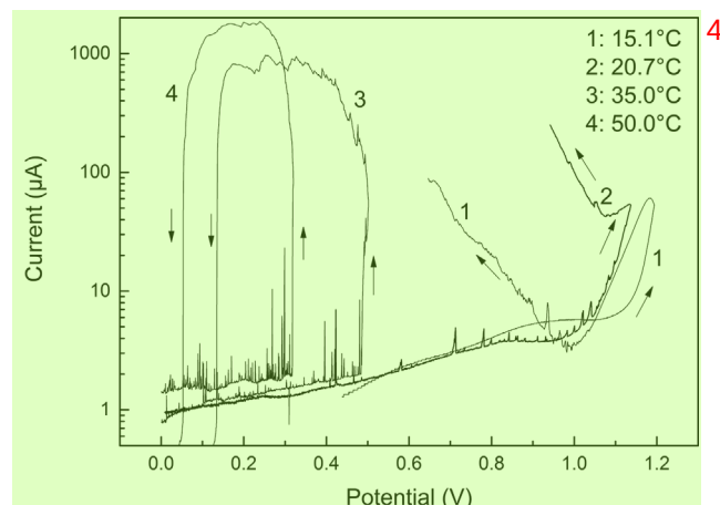
FIGURE 4 Typical cyclic polarization curves of 317L at different temperatures
