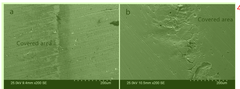
FIGURE 13 SEM morphologies of 904L after potentiostatic polarization test: (a) 950 mV and (b) 1200 mV 5
